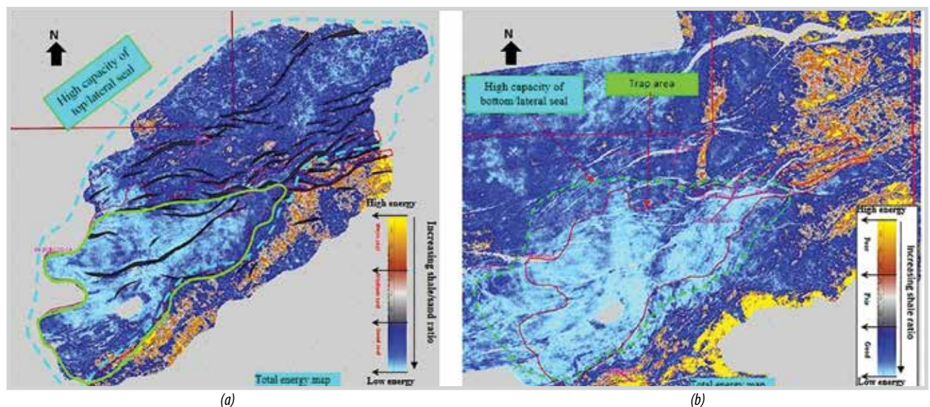
Figure 8. Sealing capacity prediction for top seal (a) and bottom/lateral seal (b) for the stratigraphic fan trap in Block 09-2/09 using seismic attribute analysis. Both seismic attribute maps show that there is high possibility of shale distributions over the trap area represented by low total energy anomalies.
