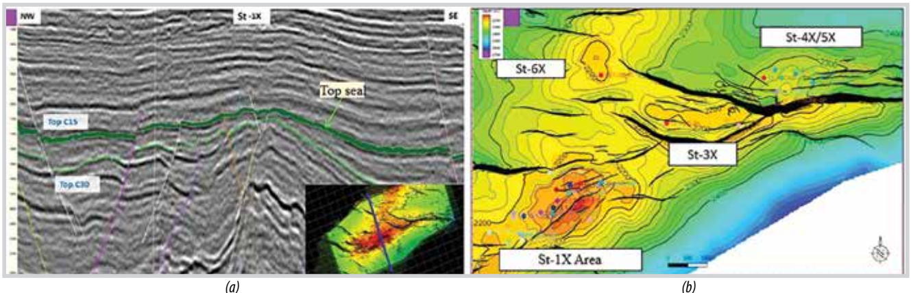
Figure 4. Seismic section through an anticline formed by post-depositional tectonics (a); Depth map of a structural trap showing four-way closure (b).
