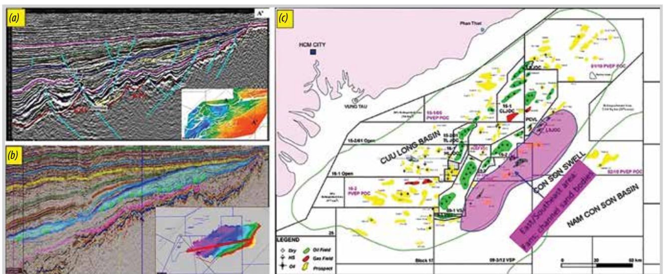
Figure 9. Possible distribution of stratigraphic traps in southeastern margin of Cuu Long basin. NW-SE seismic section showing progradation of reflections toward the basin centre (a); E-W section showing seismic characteristics that could be related to prograding deltaic depositions (b); Predicted distribution of fan-shaped traps in Oligocene section of Cuu Long basin (c).
